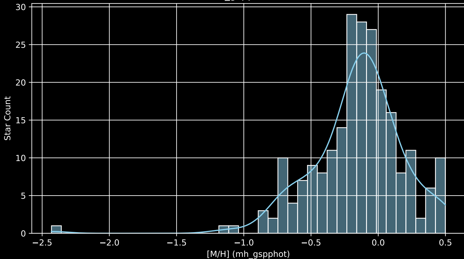
APOGEE DR17 Field: [148+31_btx [M/H] (mh_gspphot) (n= 227)
