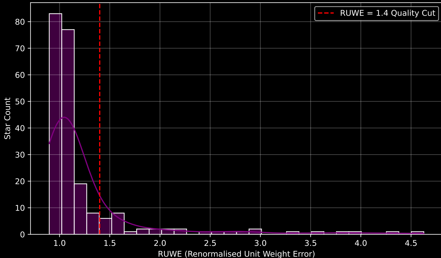
GAPOGEE DR17 Field [148+31_btx] RUWE Distribution (n= 222)
