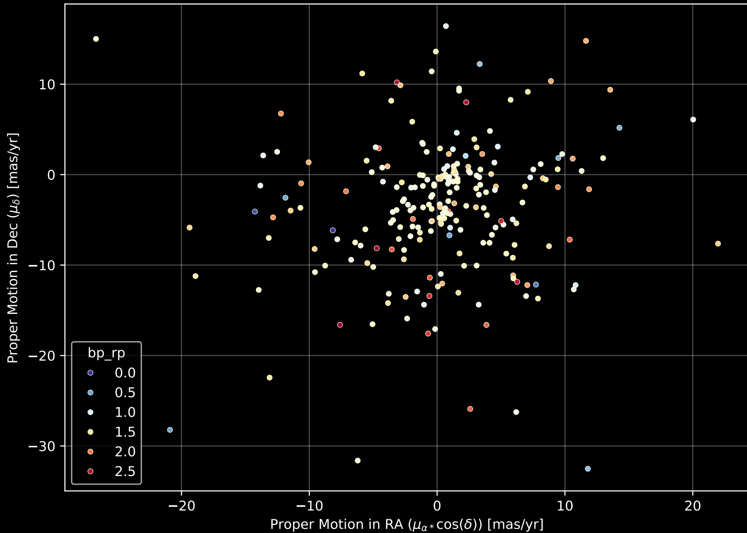
APOGEE DR17 Field: [148+31_btx] Proper Motion Diagram (n= 231)
