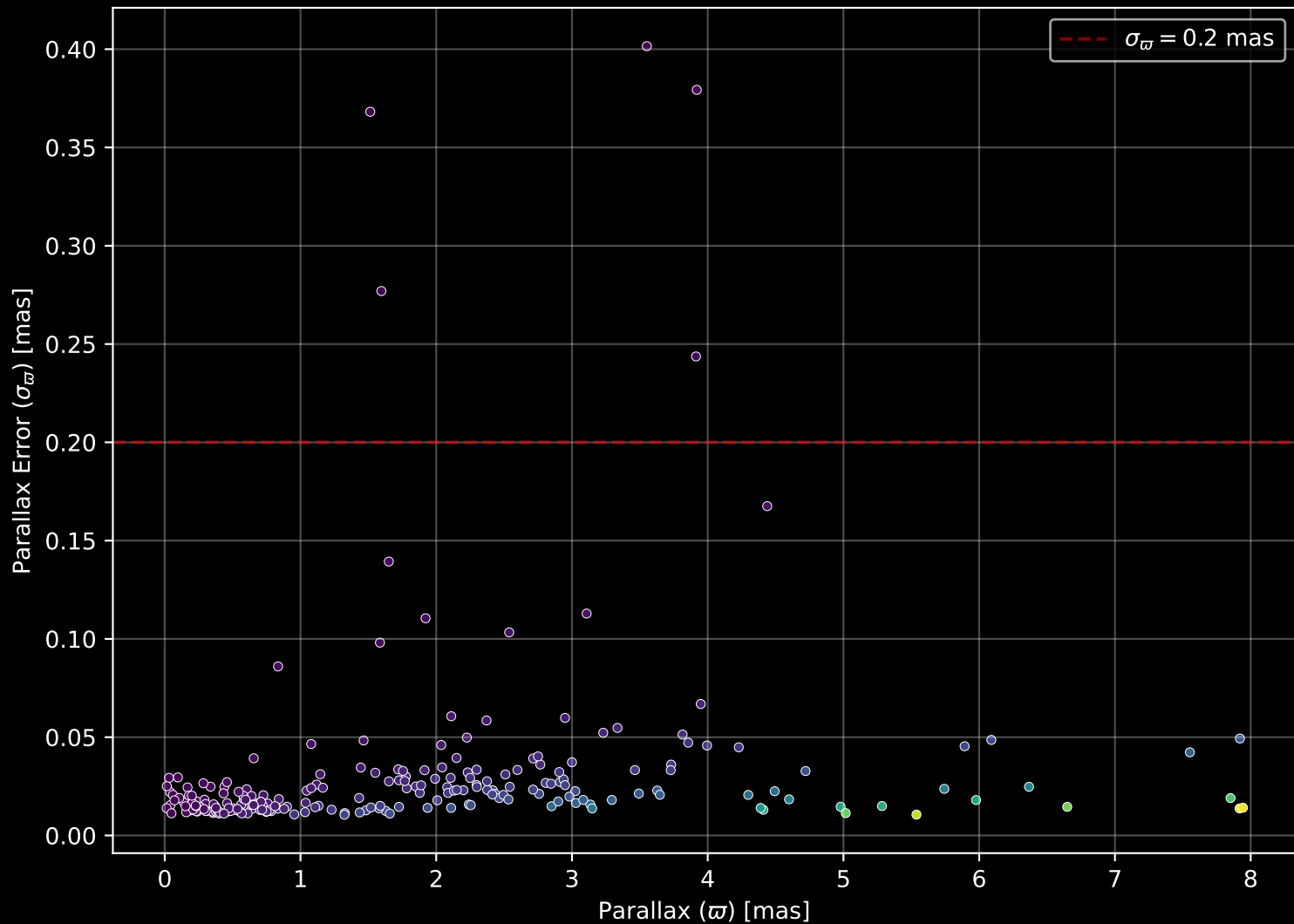
APOGEE DR17 Field: [148+31_btx] Parallax Quality (n= 231)
