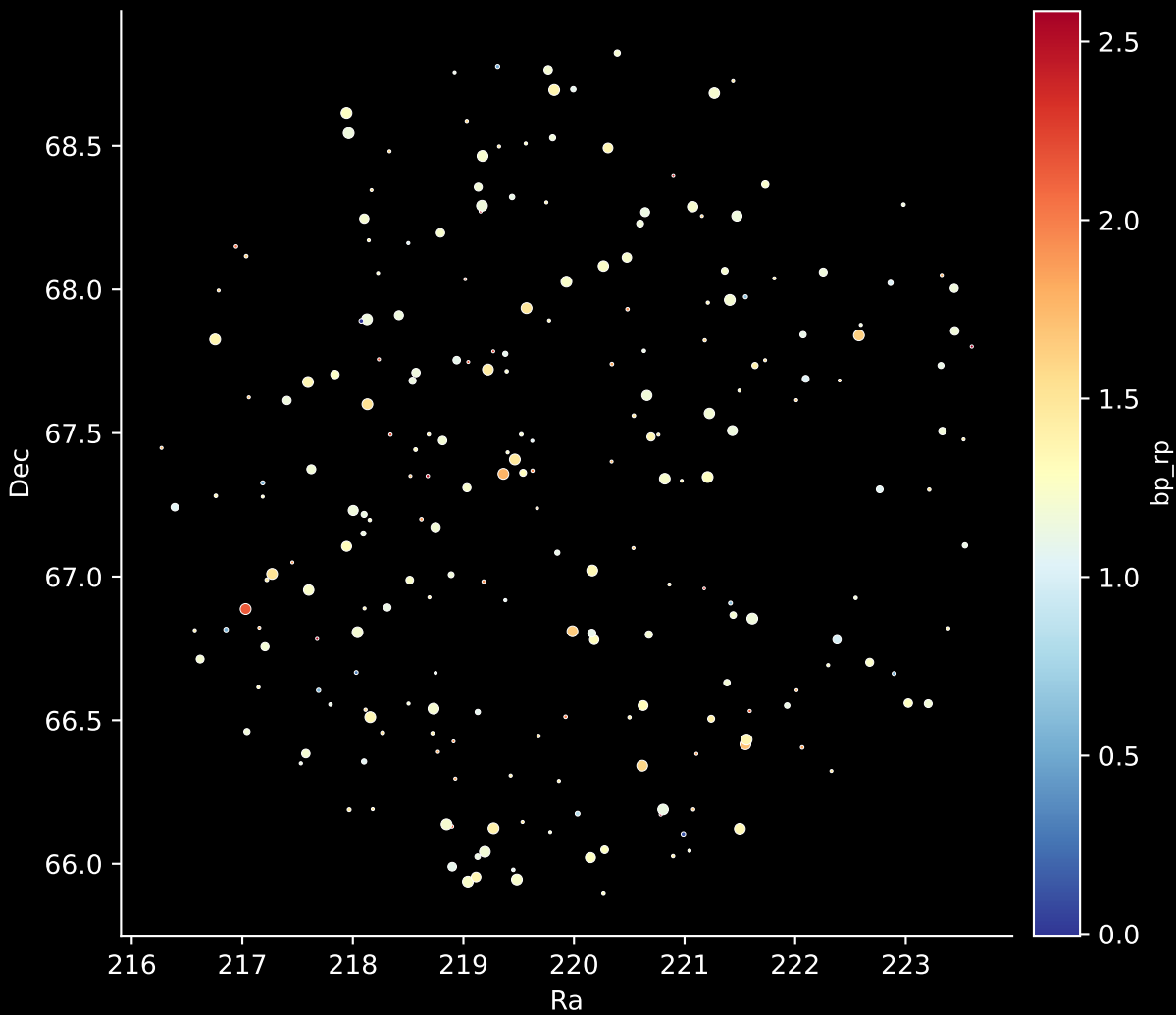
APOGEE DR17 Field: [148+31_btx] Stars: 231
