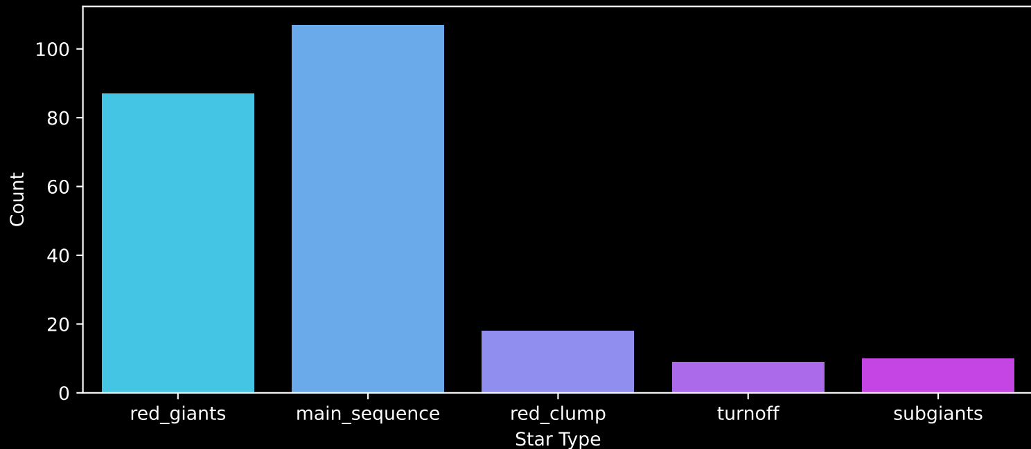
APOGEE DR17 Field: [148+31_btx] Count plot of Star Type
